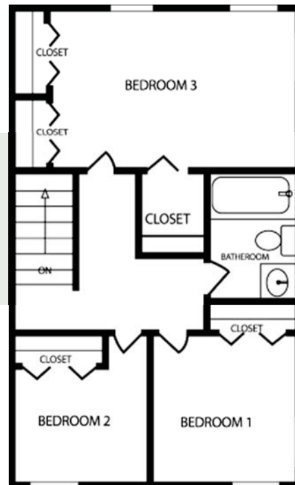
3 Bedroom / 1.5 Bath
